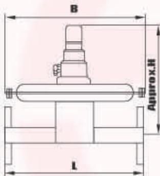
MODEL - SNB110
