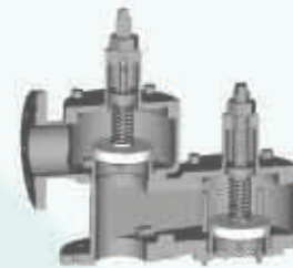
SBB, Dual Spring Loaded Type
